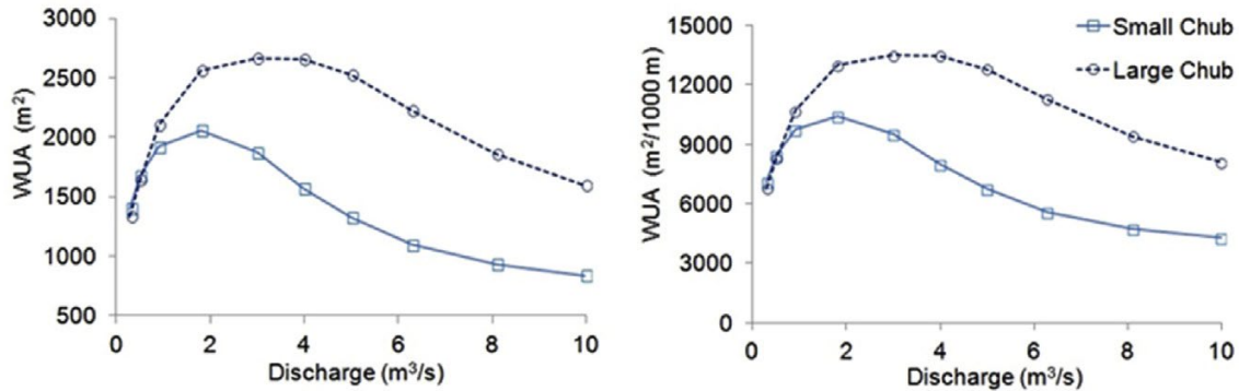
Fig. 1 Indicative WUA - Q curve (Stamou et al., 2018).
